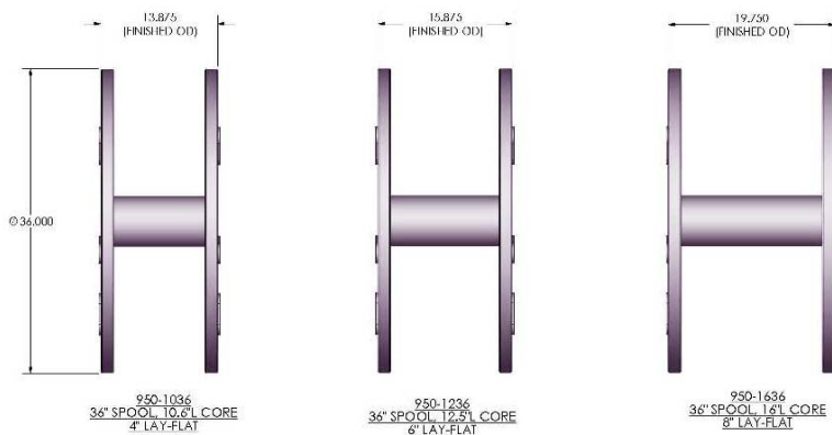
Typical method of storage. Retrieving on the layflat spool. Layflat Spool sizes: 4”, 6”, & 8”
